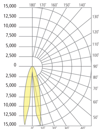
Light Distribution Curve 40°
