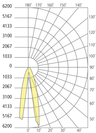
Light Distribution Curve 24°
