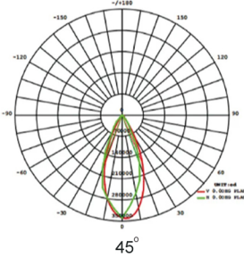
Luminous Intensity Distributin Diagram
