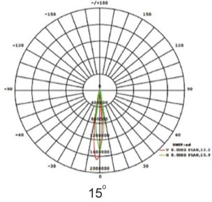
Luminous Intensity Distributin Diagram
