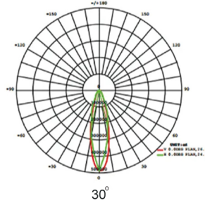
Luminous Intensity Distributin Diagram
