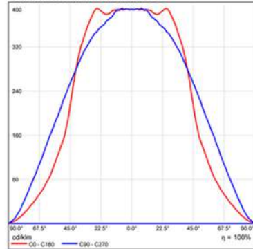
Luminous emittance 1 / Linear LDC
