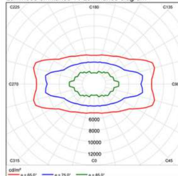
Luminous emittance 1 / Luminance diagram
